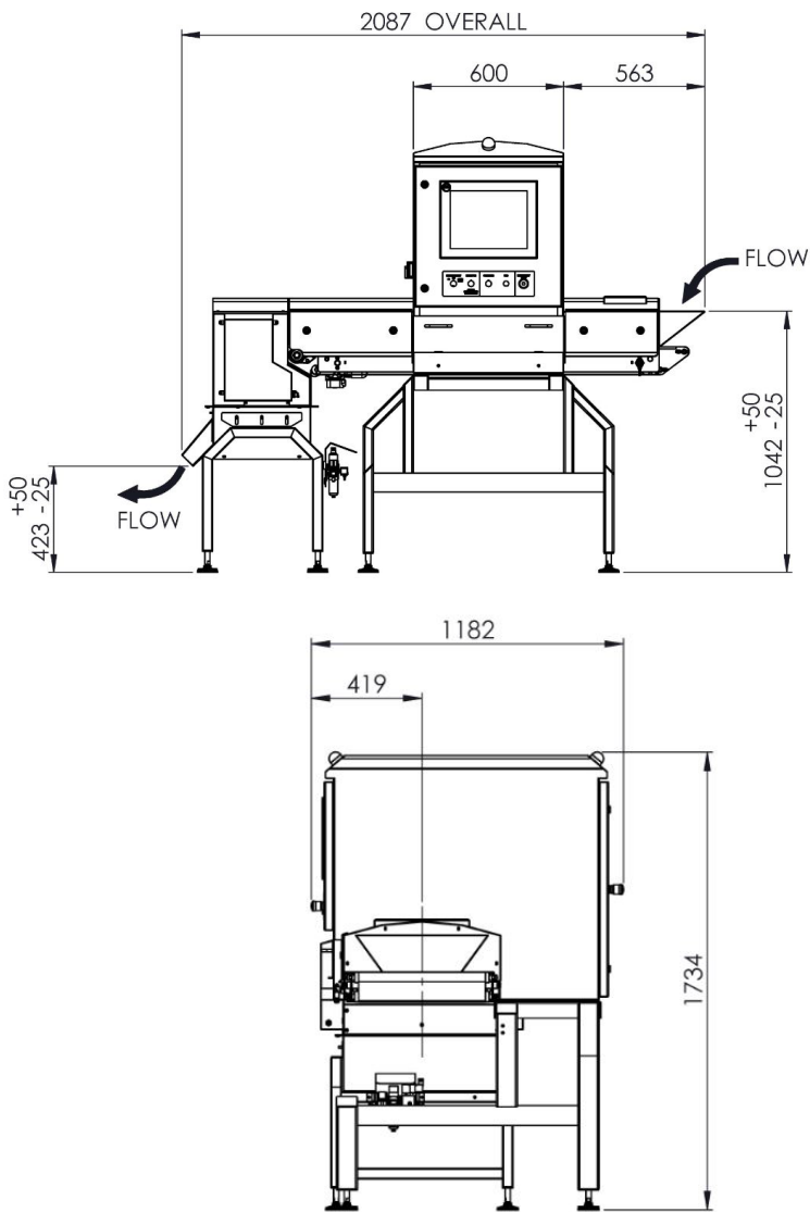
Typical system dimensions shown (in mm). Dimensions are dependent on system configuration.
